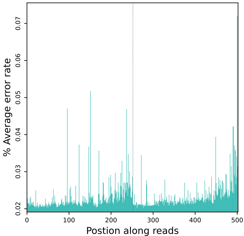
Error rate distribution along reads (R20213)
